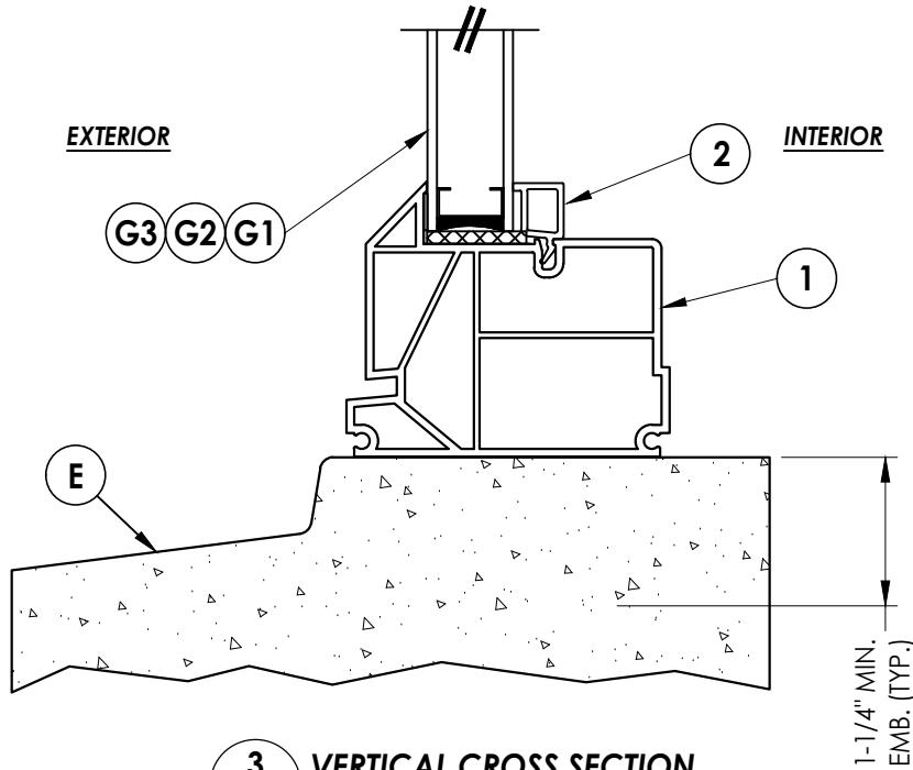
3 VERTICAL CROSS SECTION 3 Optional masonry sill
